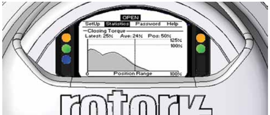
A diagnostic screen display, showing torque and position data in real time
